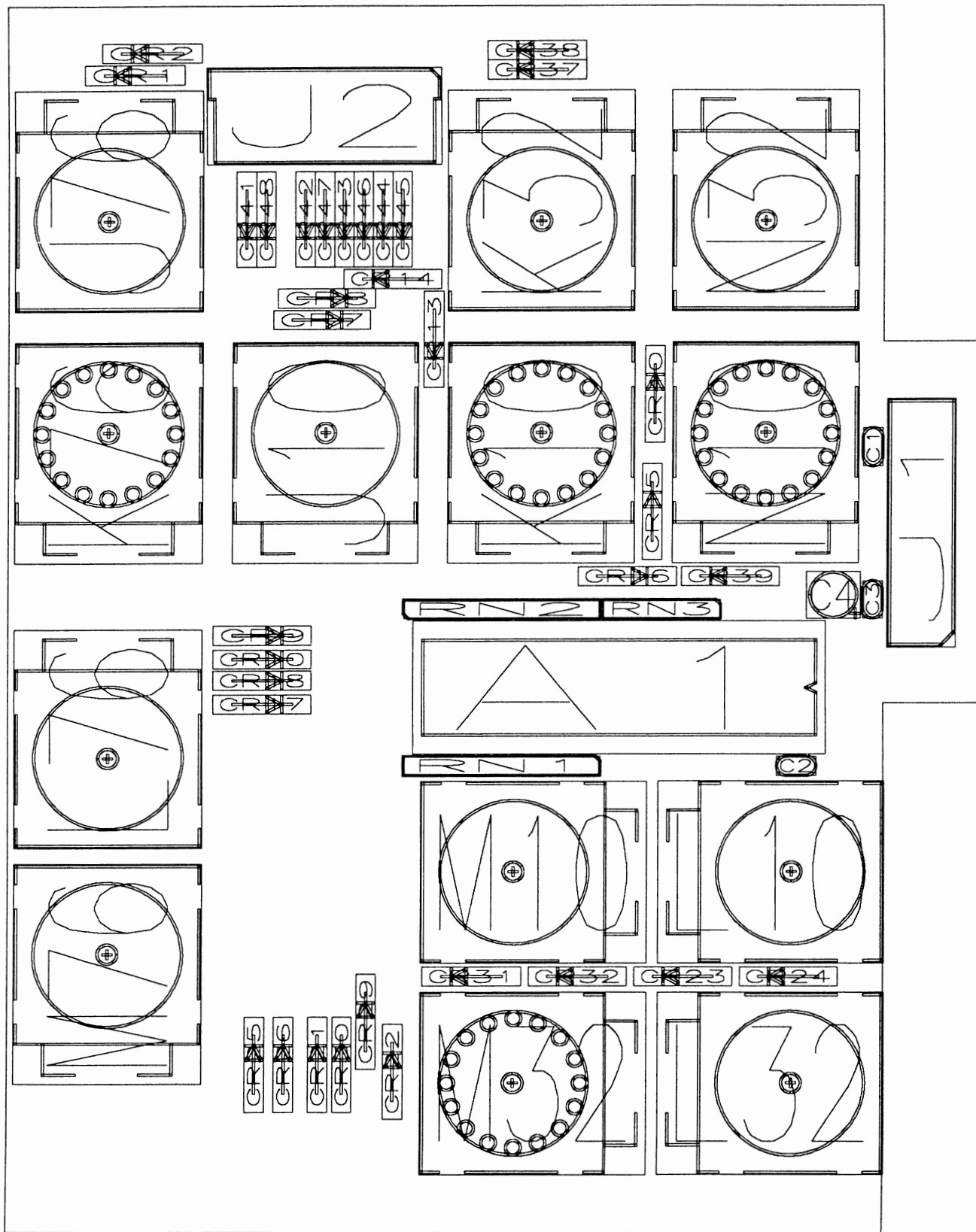
9300-5 PCB Rev: A
